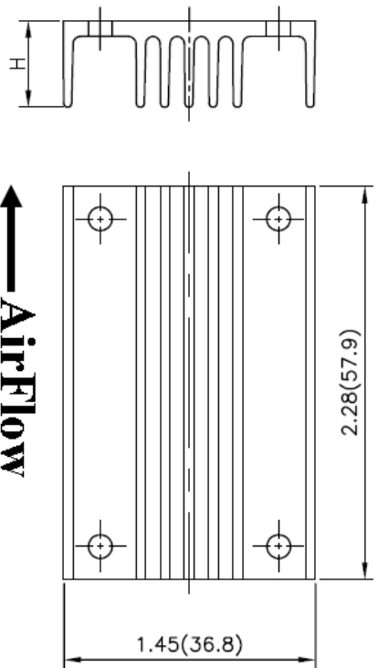
Vertical Fin Orientation, Suffix:-HS2, -HS3
