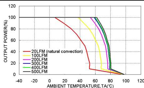
QAE150-48S05 Derating Curve With 0.24" Height Heat-sink
