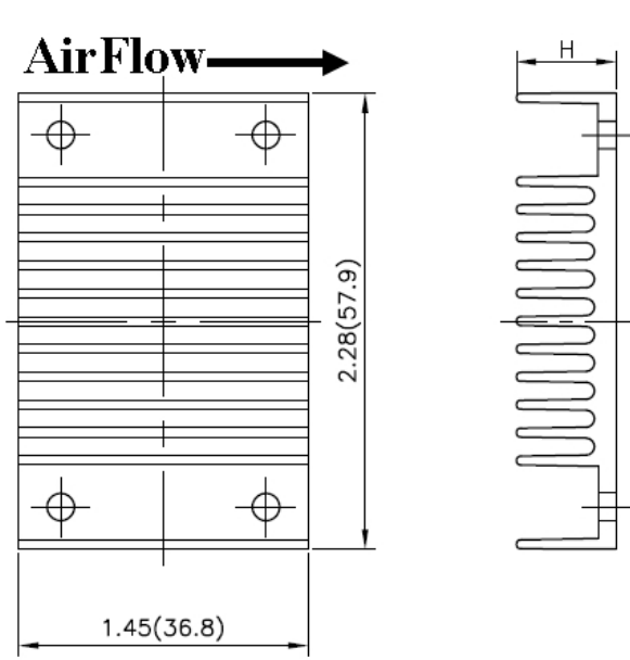
Horizontal Fin Orientation, Suffix:-HS, -HS1
